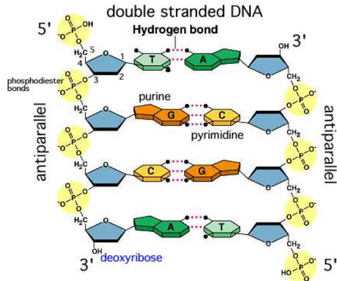
Figure 2.5: Double-stranded DNA. (from City University of New York) The 5' end and the 3' end refer to the two distinctive ends of DNA.
