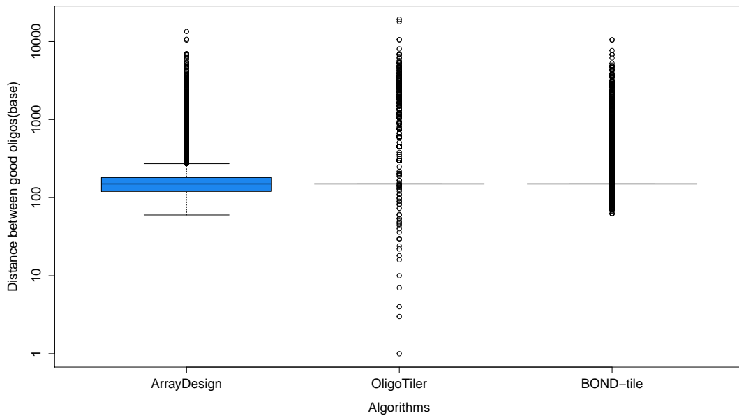
Distance of good oligos (T.reeseiV2 dataset)
