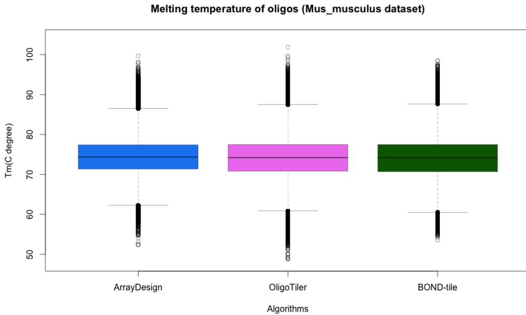
Figure 4.13: Melting temperature distribution for the Mus musculus dataset.
